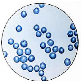
Coccus – 1 mcm
