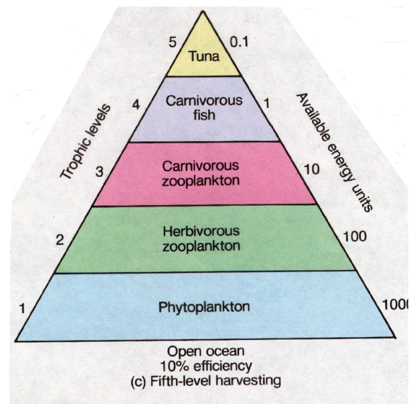
Energy Pyramid
